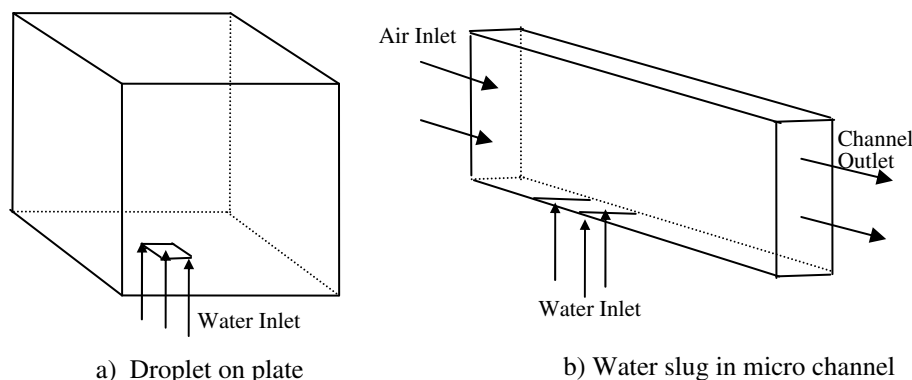
Fig. 7. Sketch of calculation domain and boundaries (not drawn to scale).
